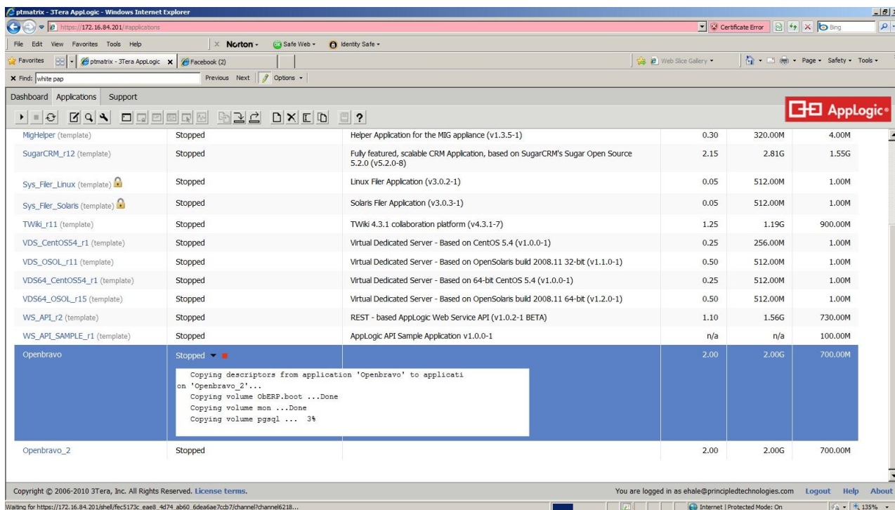
Figure 8: CA 3Tera AppLogic in the process of copying the Openbravo application.
